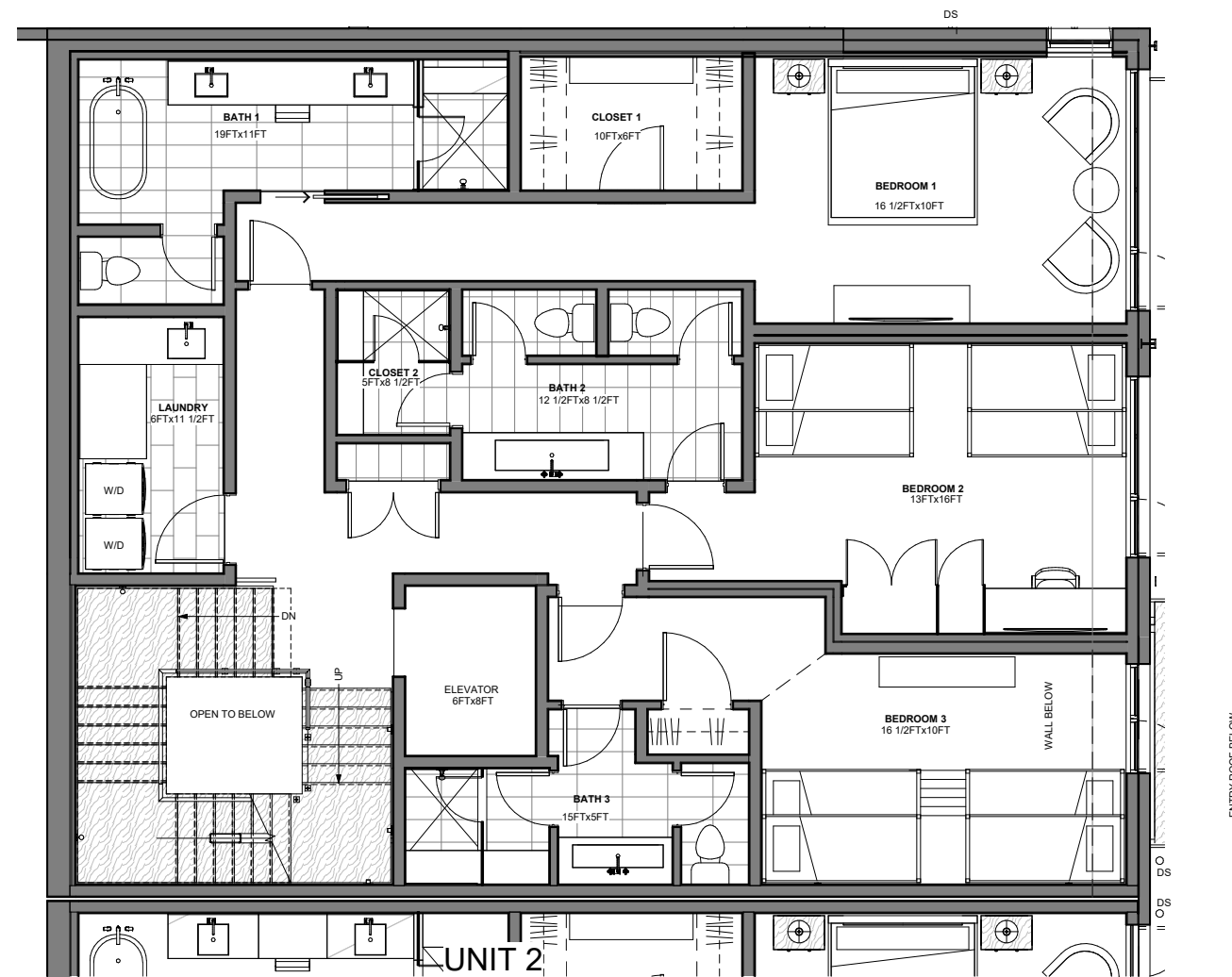
② UNIT 1 - FIRST STORY-MARKETING 1/4" = 1'-0"
